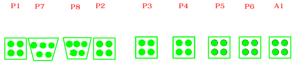
PILE FOUNDATION
